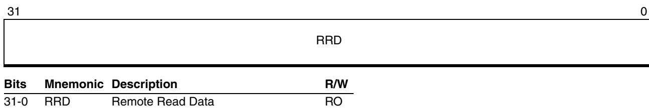
Figure 16-18. Remote Read Register (APIC Offset C0h)
