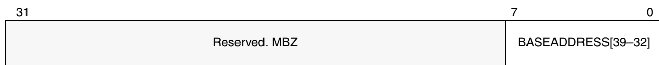
Figure 15-8. Format of DEV_BASE_HI[n] Registers
