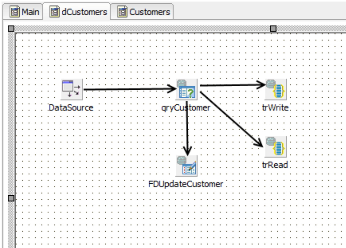
Figure 5. dCustomers datamodule
