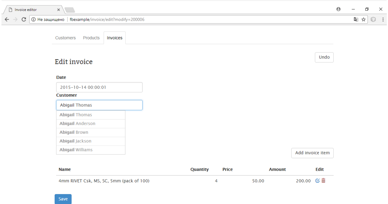
Figure 42. Invoice editor
