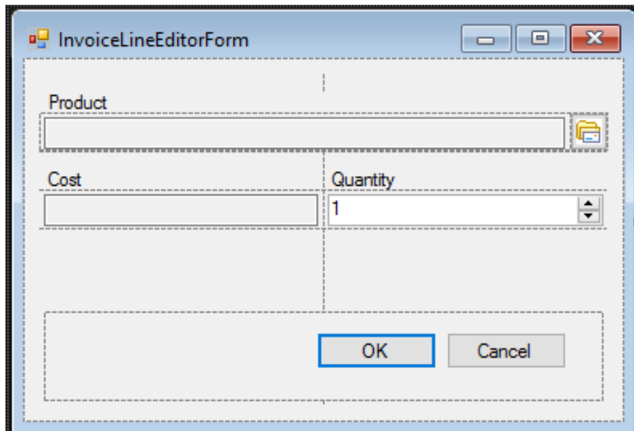
Figure 27. Product form
