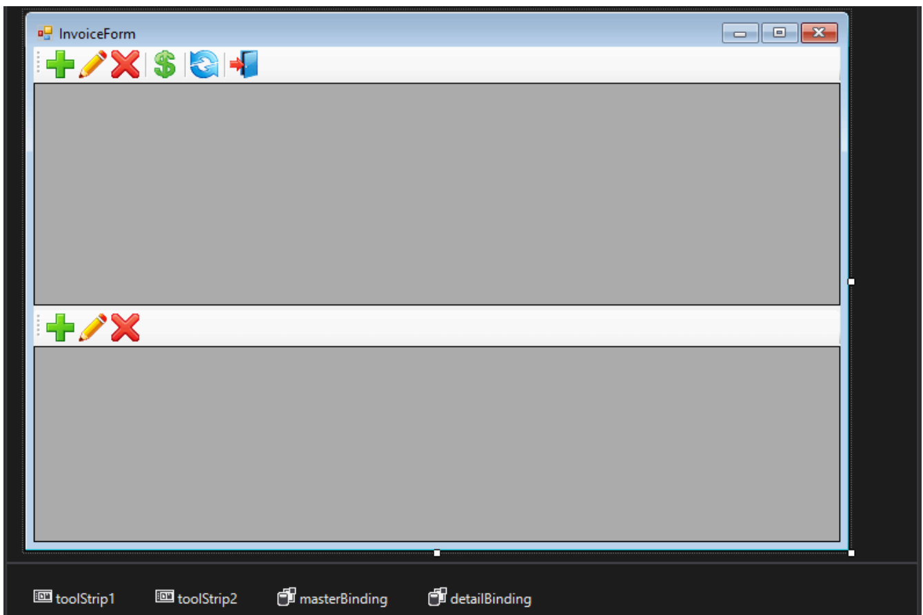
Figure 26. Invoice form
