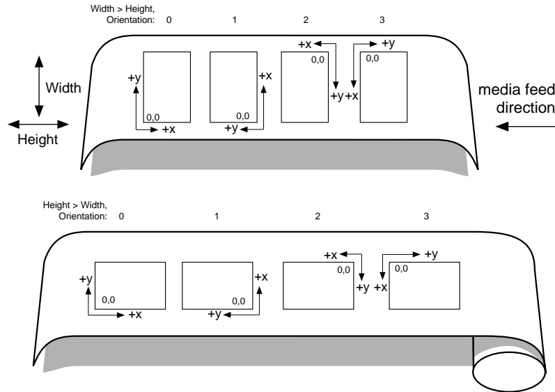
Figure 2 Roll-fed media devices
